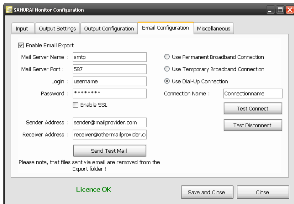
Figure 2: E-mail configuration
