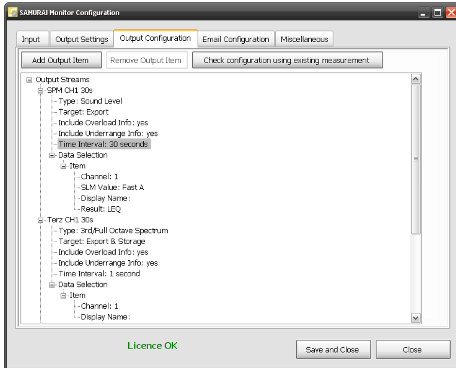
Figure 1: Export configuration
